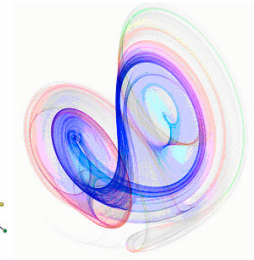
The Lorenz attractor
